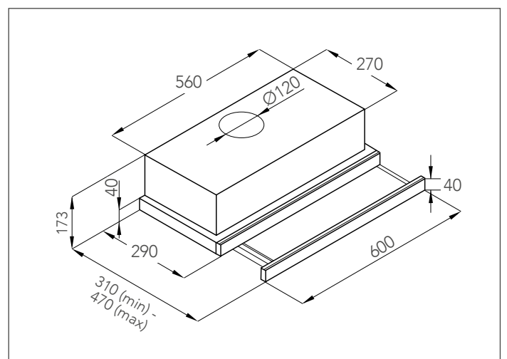
SCRH60 SLIDE-OUT RANGEHOOD // 60cm
