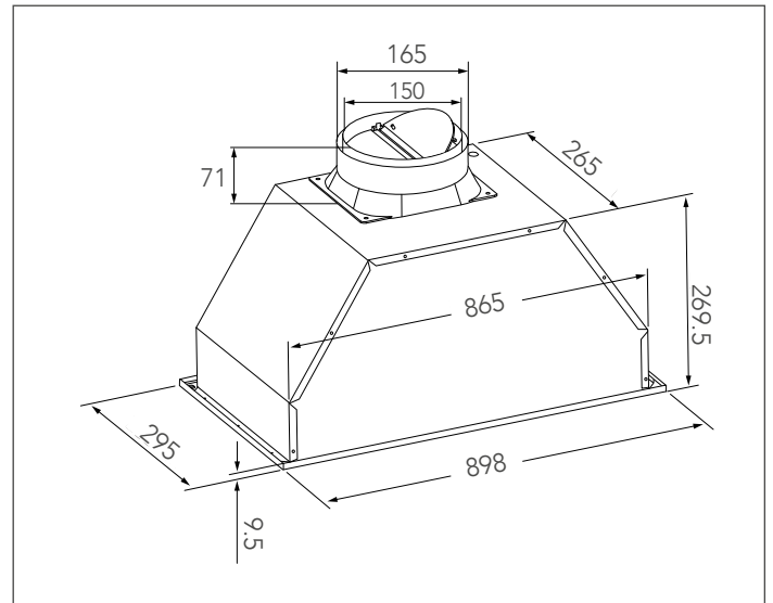
SCUM-9C UNDERMOUNT RANGEHOOD // 90cm
