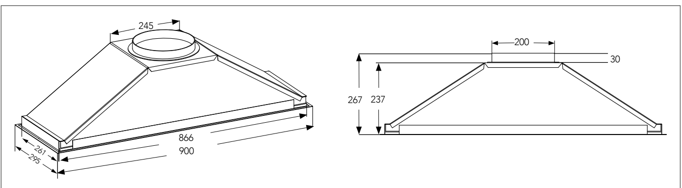
SC900UMS UNDERMOUNT RANGEHOOD / SILENT // 90cm
