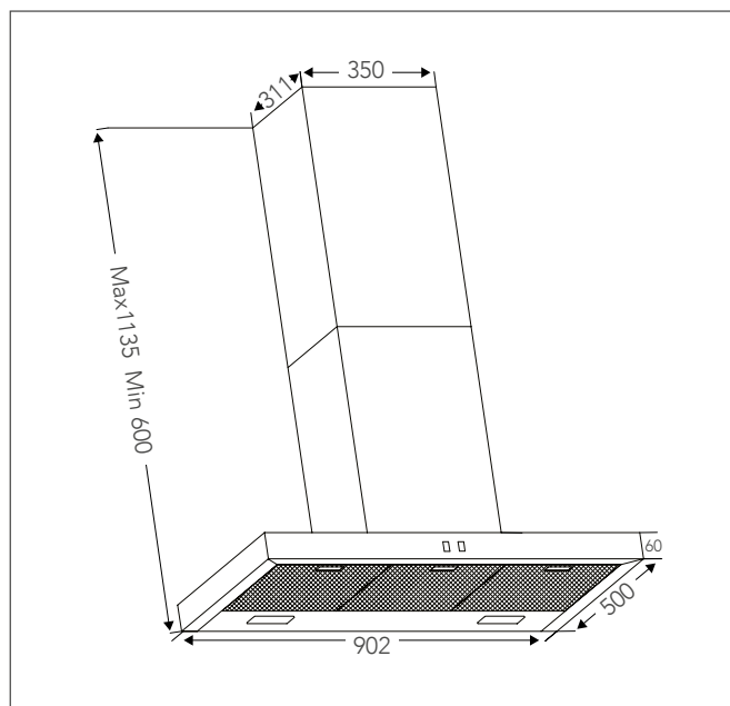
SC900WTS, SC900WRS WALLMOUNT RANGEHOOD / SILENT // 90CM
