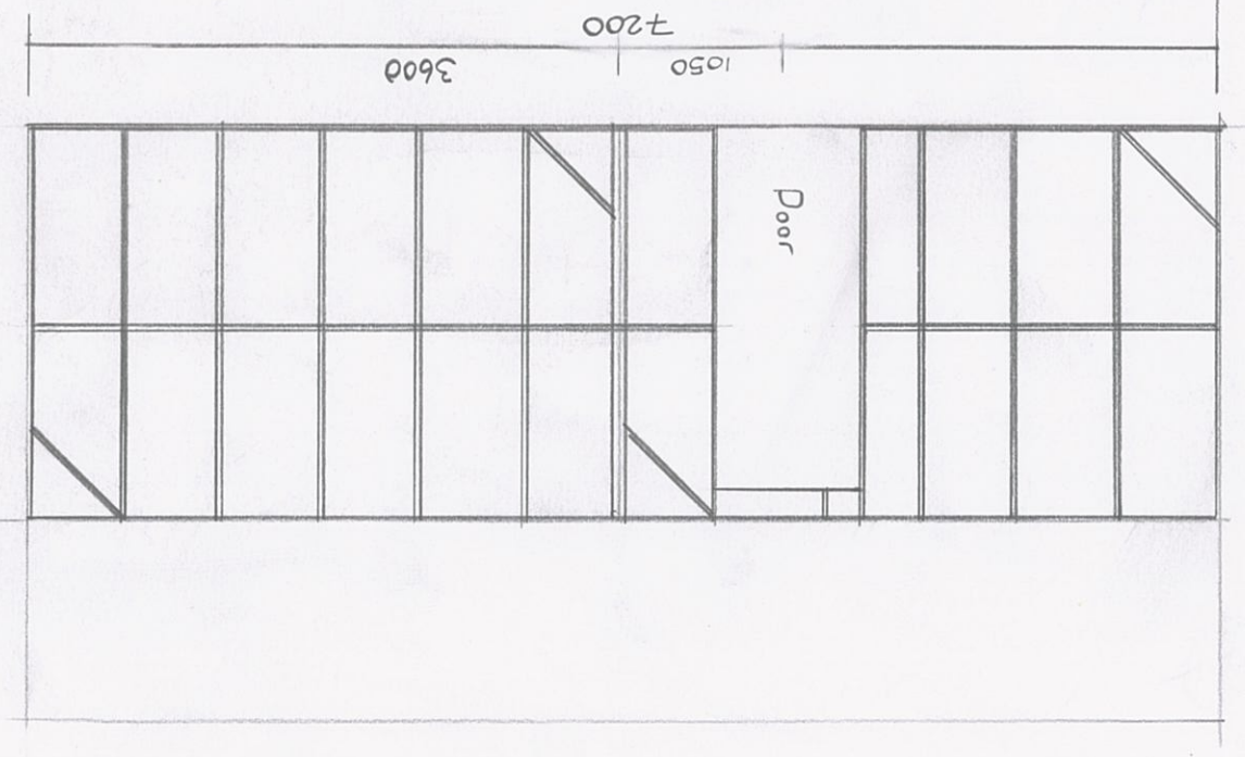
External Wall - South Elevation
